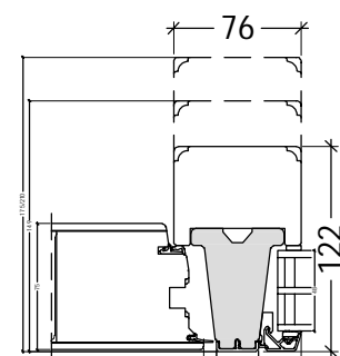
V3: FRAic24-50L48 V6: FRAic24-50L48(mirr.)
