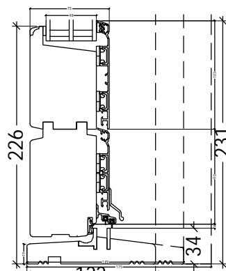
L2: FRAic22-11L48
