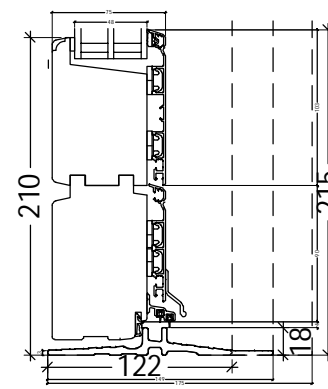
L2: FRAic22-13L48
