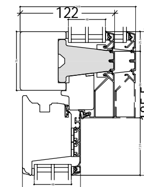
L6: FRAic23-41L48
