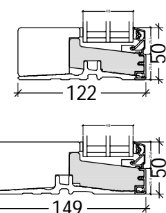
L4: FRAic23-10L48
