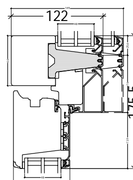
L6: FRAic23-40L48
