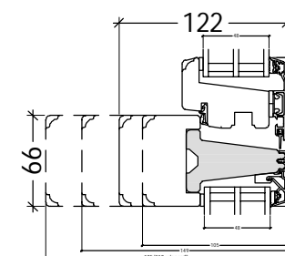
L3: FRAic06-20L48
